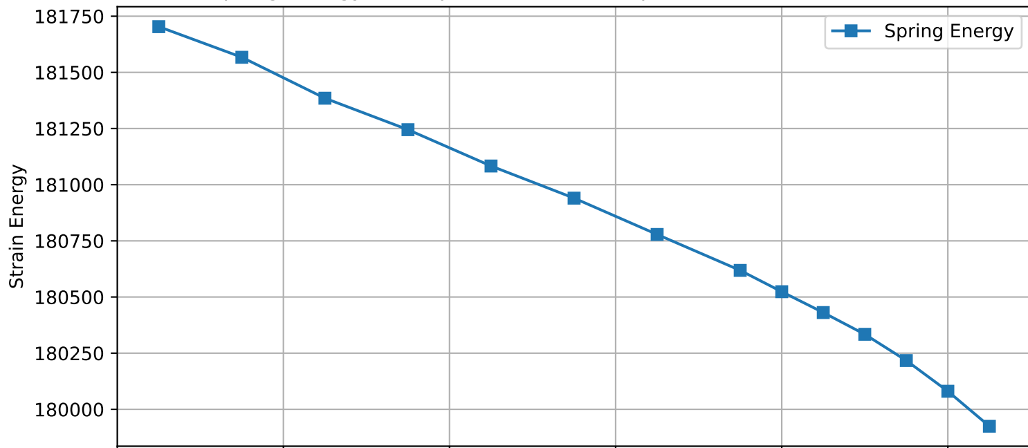
Spring Energy vs. Rupture Position, Displacement Control, 4.0MPa
