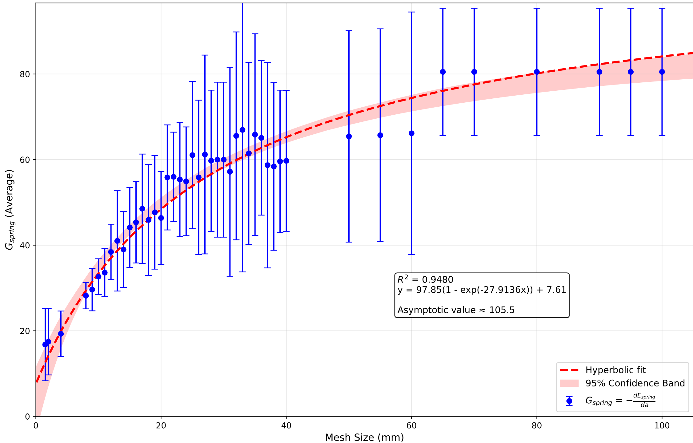
Best Fit (Hyperbolic) of Average Spring Energy Gradient vs. Mesh Size Displacement Control
