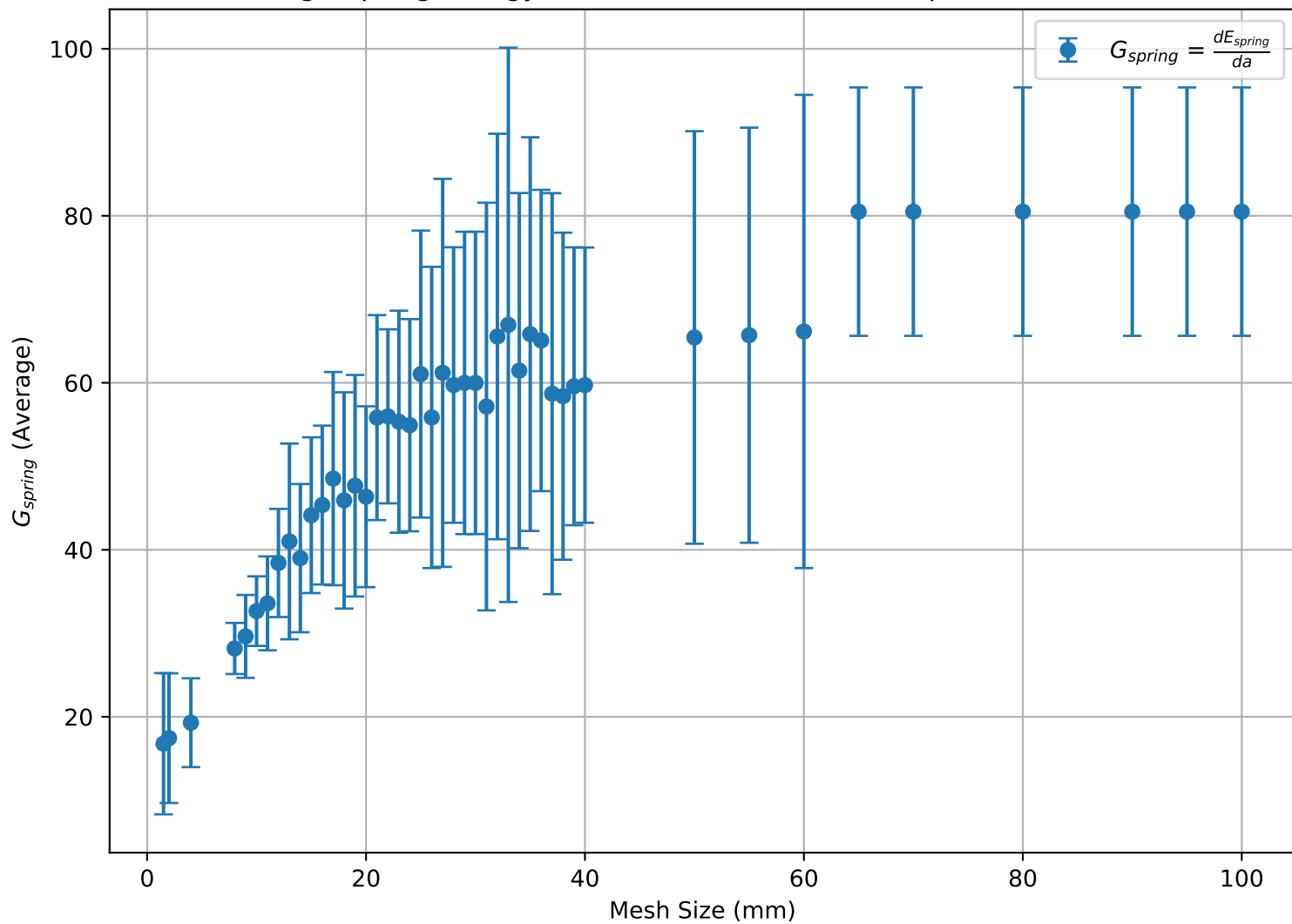
Average Spring Energy Gradient vs. Mesh Size, Displacement Control
