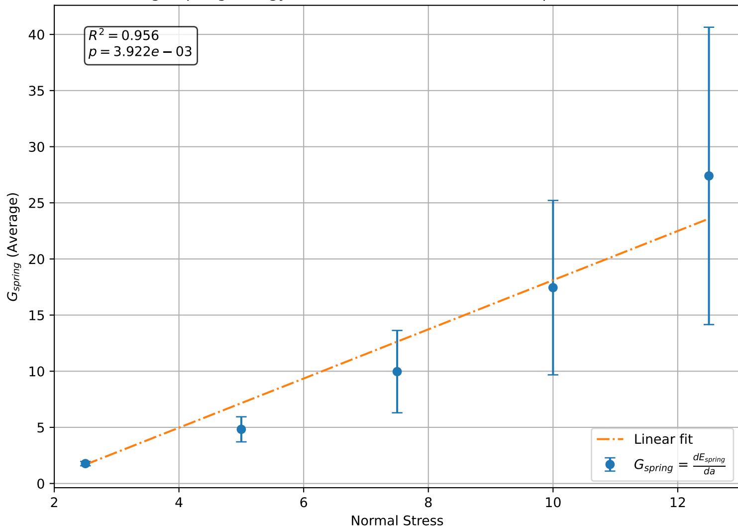
Average Spring Energy Gradient vs. Normal Stress, Displacement Control
