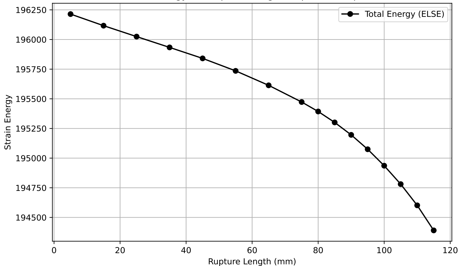
Strain Energy vs. Rupture Length (Top-down Rupture)
