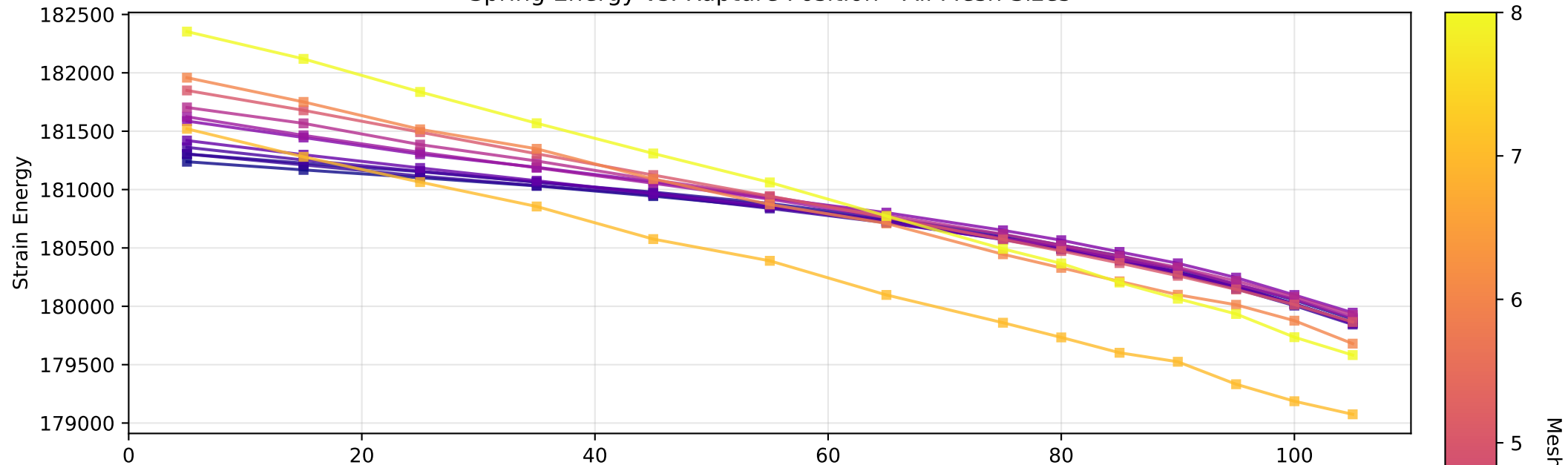
Spring Energy vs. Rupture Position - All Mesh Sizes
