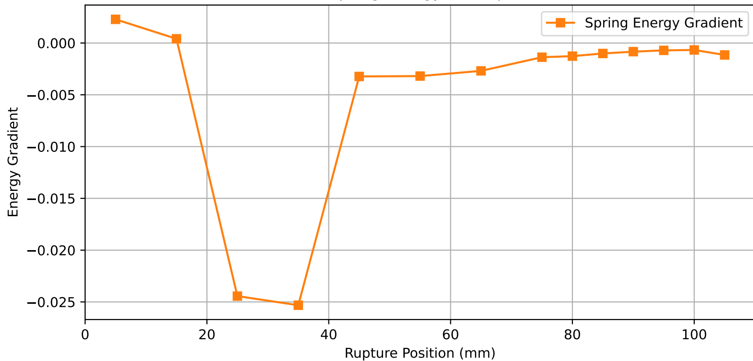
Gradient of Spring Energy vs. Rupture Position
