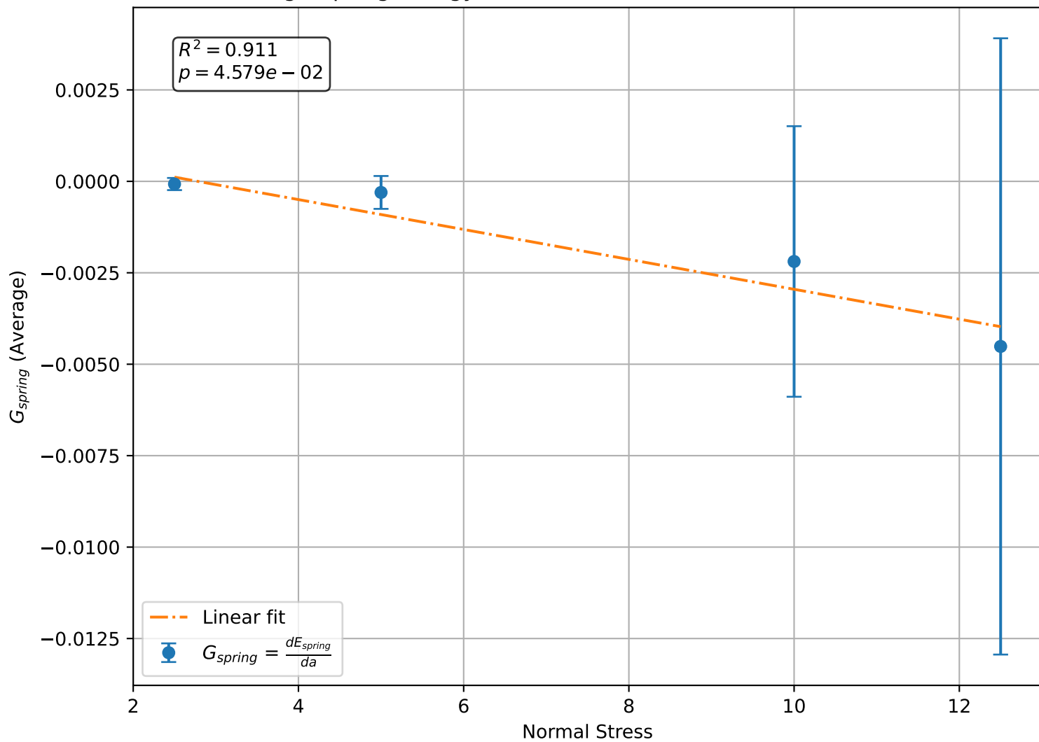
Average Spring Energy Gradient vs. Normal Stress, Stress Control
