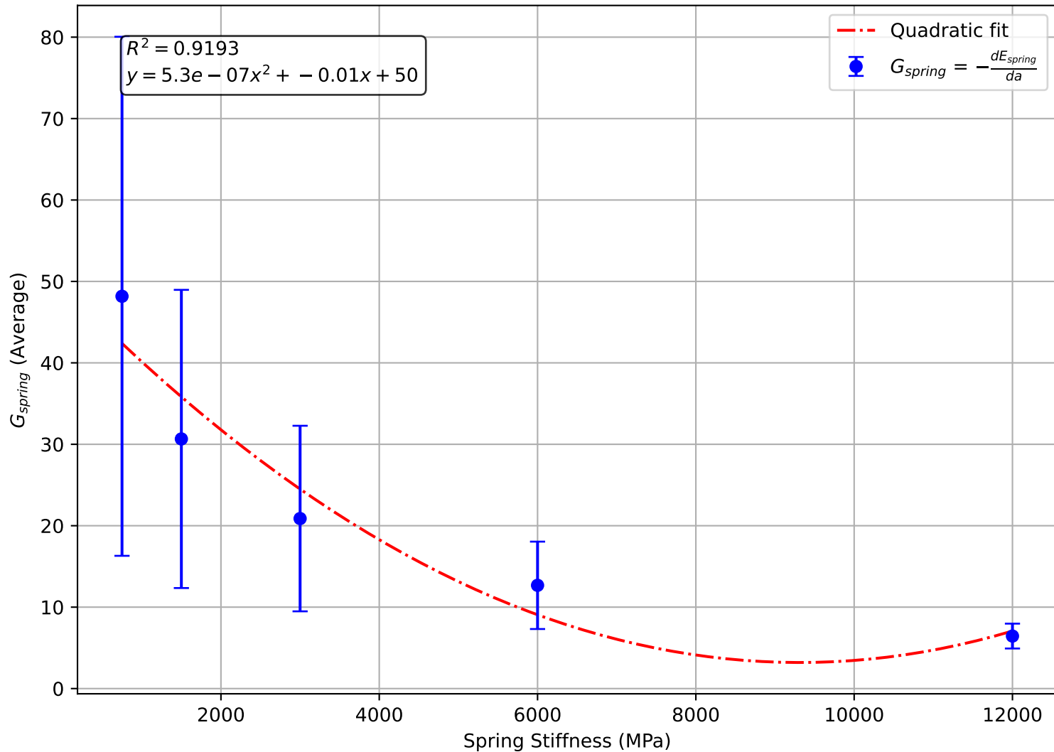
Quadratic Fit of Average Spring Energy Gradient vs. Stiffness, Displacement Control
