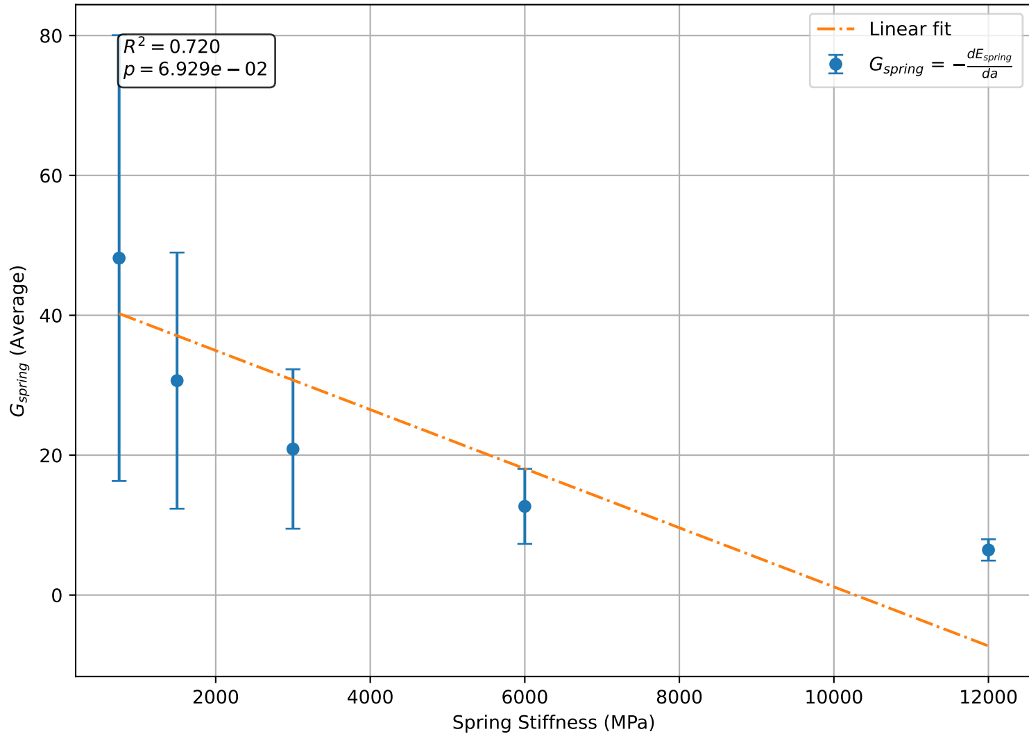
Average Spring Energy Gradient vs. Stiffness, Displacement Control
