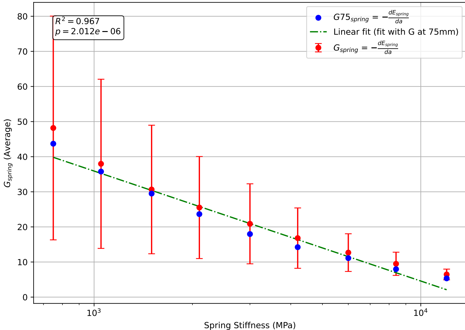
Linear Fit: Average Spring Energy Gradient (at 75mm) vs. Stiffness
