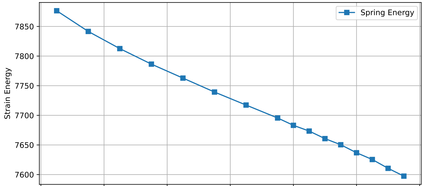
Spring Energy vs. Rupture Position, Displacement Control, E = 30000\text{MPa}
