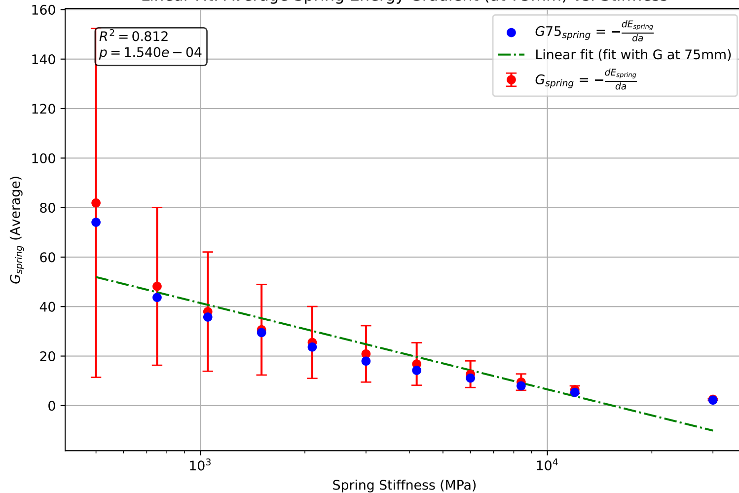
Linear Fit: Average Spring Energy Gradient (at 75mm) vs. Stiffness
