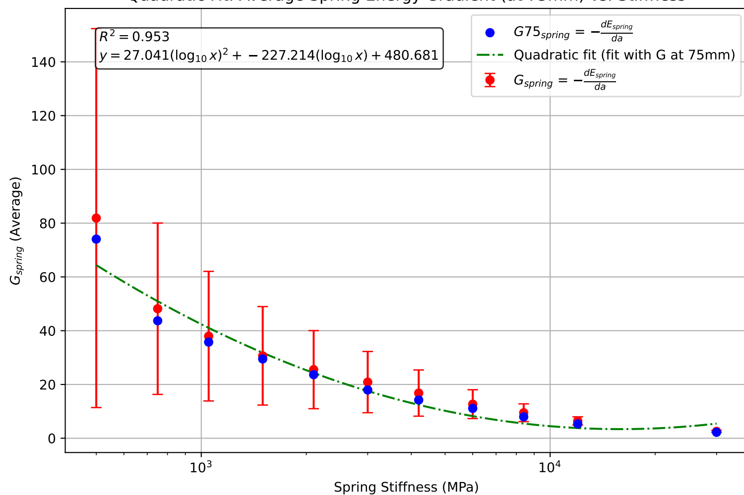
Quadratic Fit: Average Spring Energy Gradient (at 75mm) vs. Stiffness
