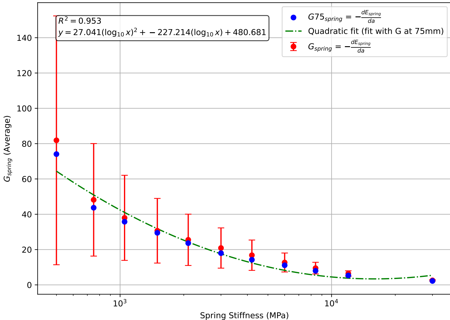
Quadratic Fit: Average Spring Energy Gradient (at 75mm) vs. Stiffness
