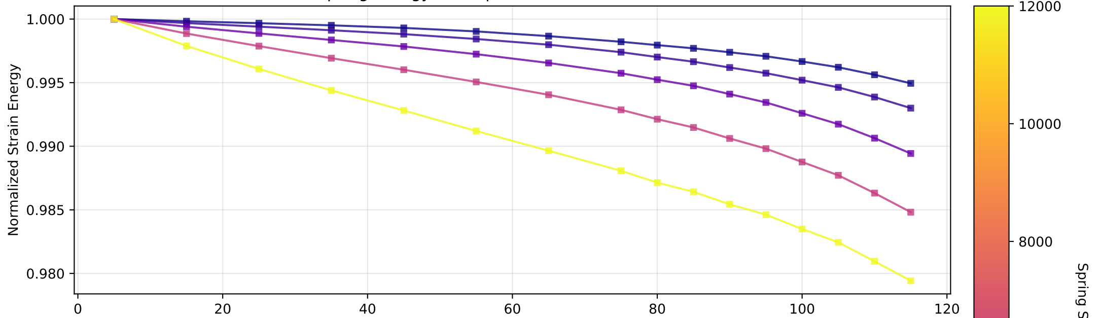
Spring Energy vs. Rupture Position - All Stiffness
