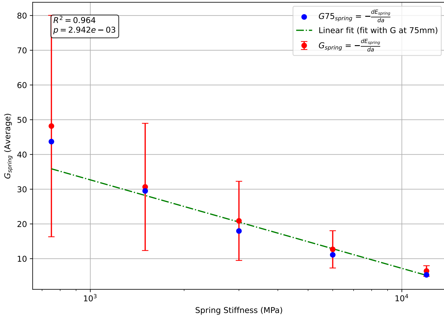
Average Spring Energy Gradient (at 75mm) vs. Stiffness, Displacement Control
