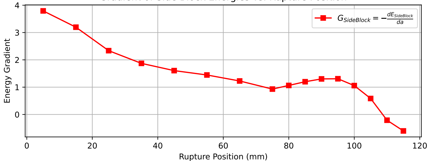
Gradient of Side Block Energies vs. Rupture Position
