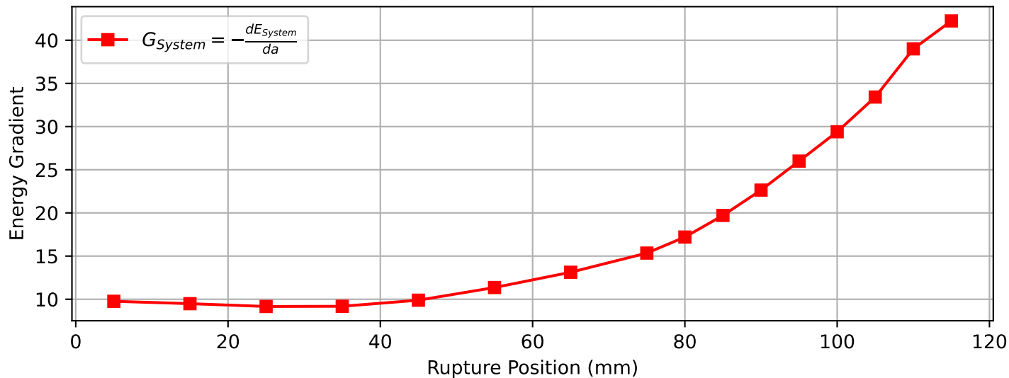
Gradient of System Energies vs. Rupture Position
