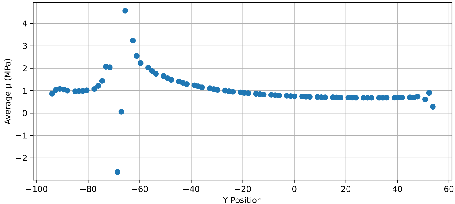
Y-direction Averaged Shear Stress \mu
