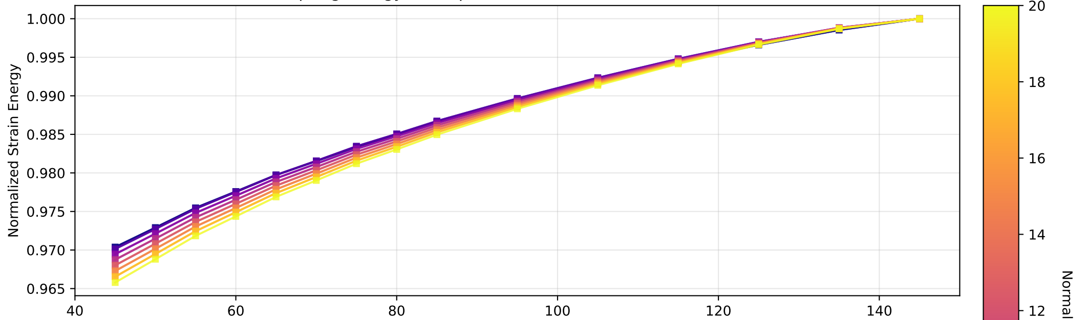
Spring Energy vs. Rupture Position - All Normal Stresses
