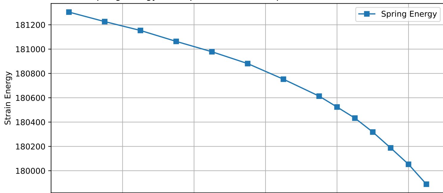
Spring Energy vs. Rupture Position, Displacement Control, 1.5MPa
