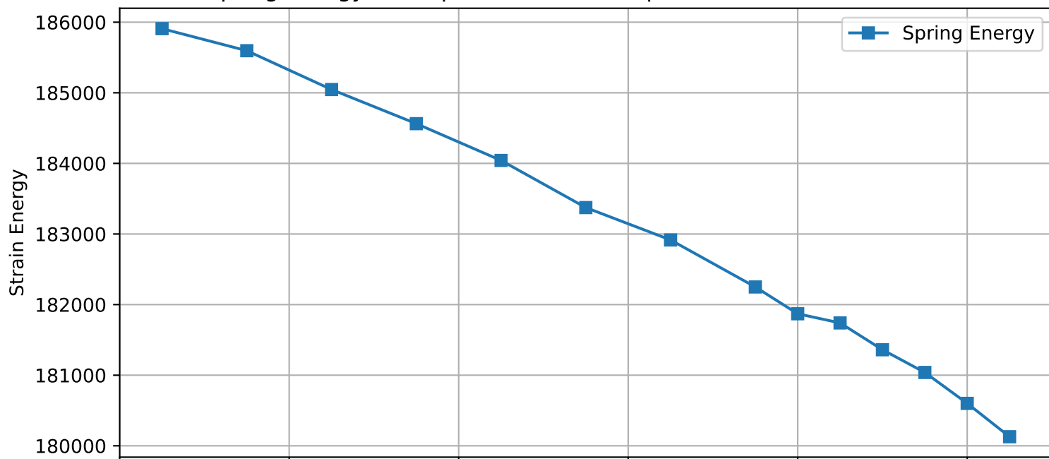
Spring Energy vs. Rupture Position, Displacement Control, 25.0MPa
