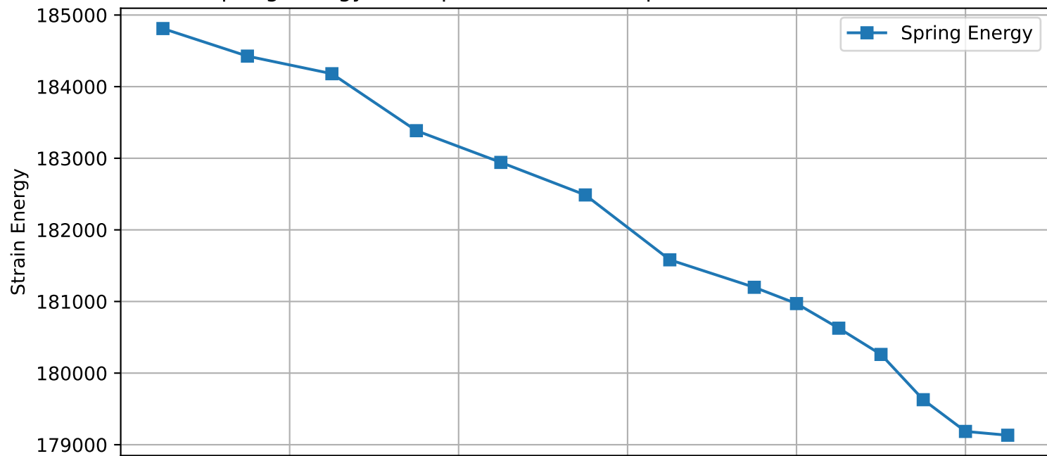
Spring Energy vs. Rupture Position, Displacement Control, 31.0MPa
