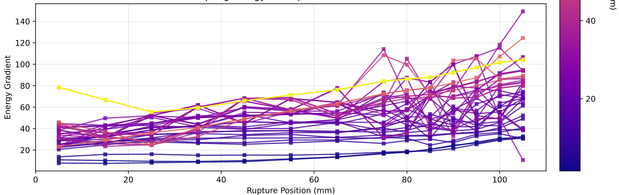
Gradient of Spring Energy vs. Rupture Position - All Mesh Sizes
