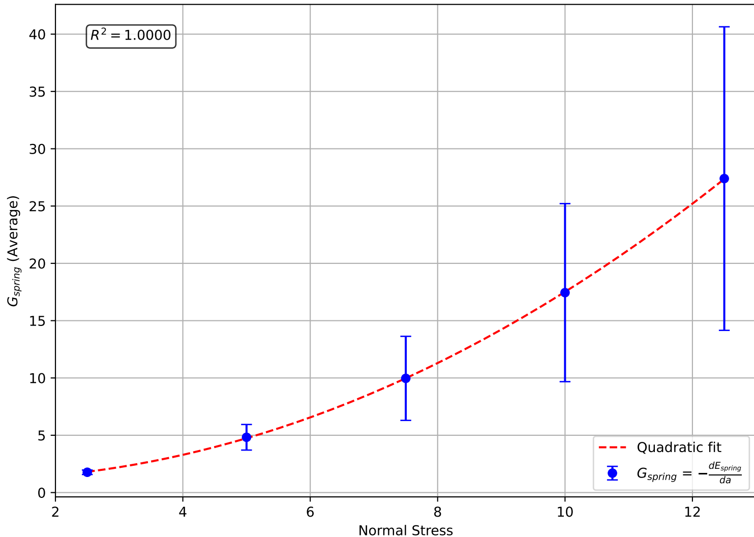
Quadratic Fit of Average Spring Energy Gradient vs. Normal Stress
