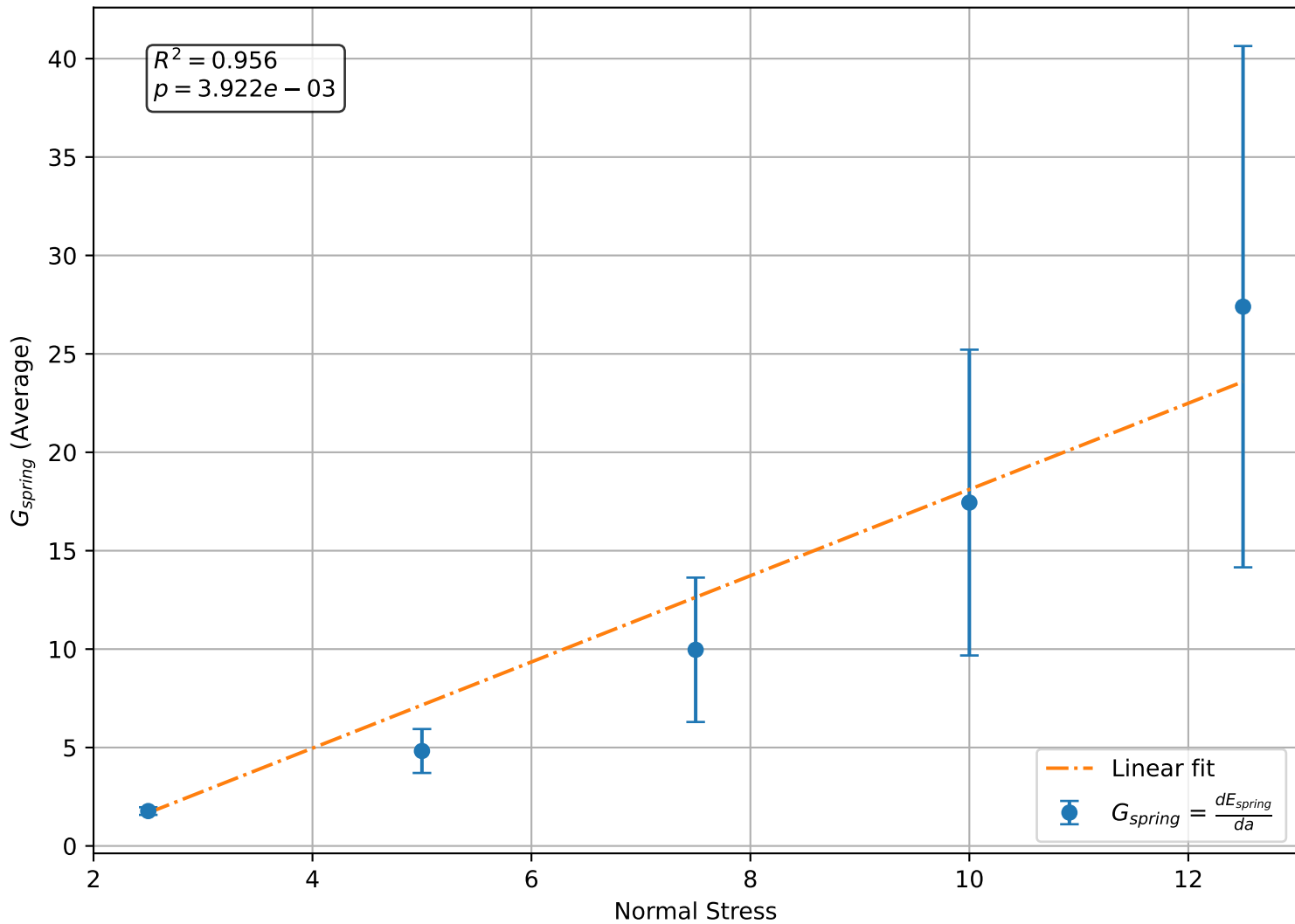
Average Spring Energy Gradient vs. Normal Stress
