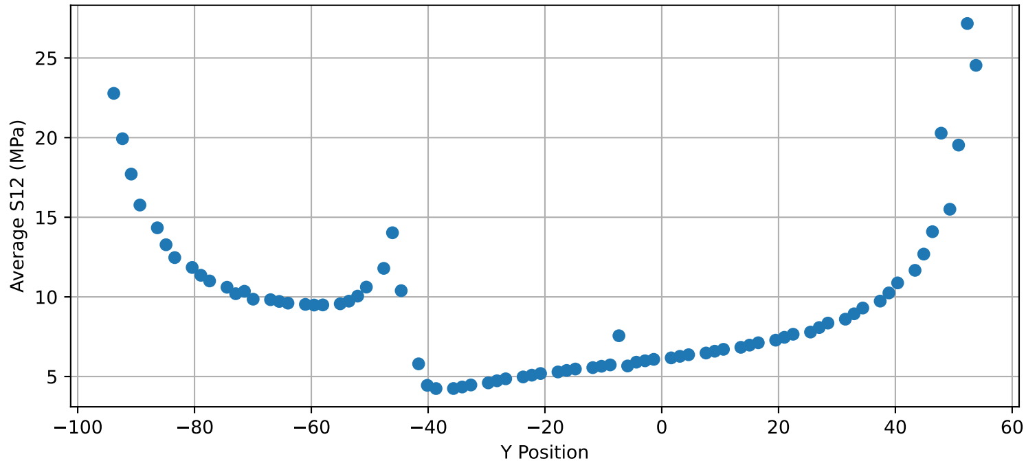
Y-direction Averaged Shear Stress S12
