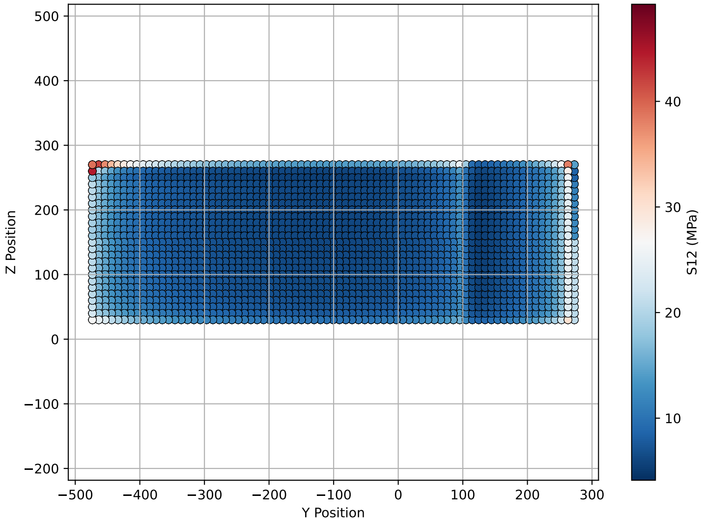
Shear Stress S12 on RIGHT-LEFT Face (YZ Projection)
