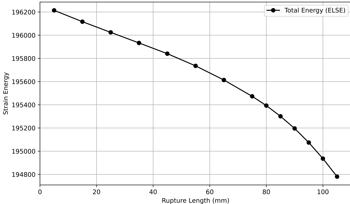
Strain Energy vs. Rupture Length (Top-down Rupture)
