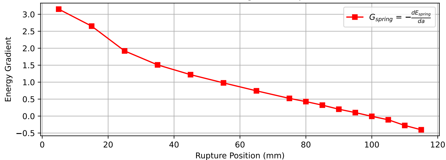
Gradient of Side Block Energies vs. Rupture Position
