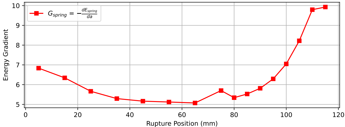
Gradient of Spring Energies vs. Rupture Position
