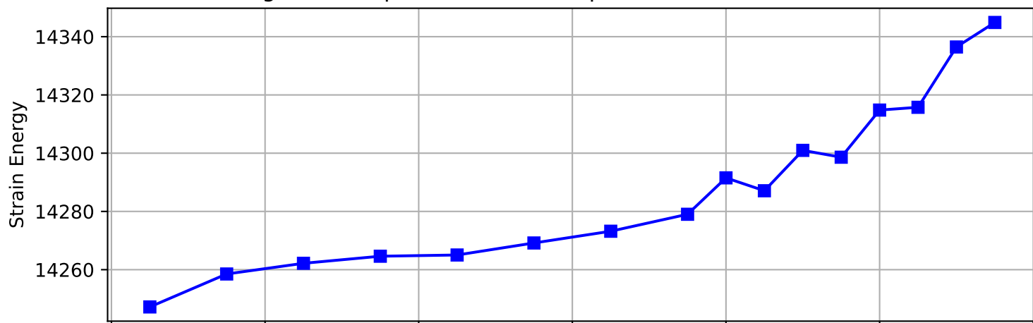
Block Energies vs. Rupture Position, Displacement Control, 10.0MPa, 2.0mm
