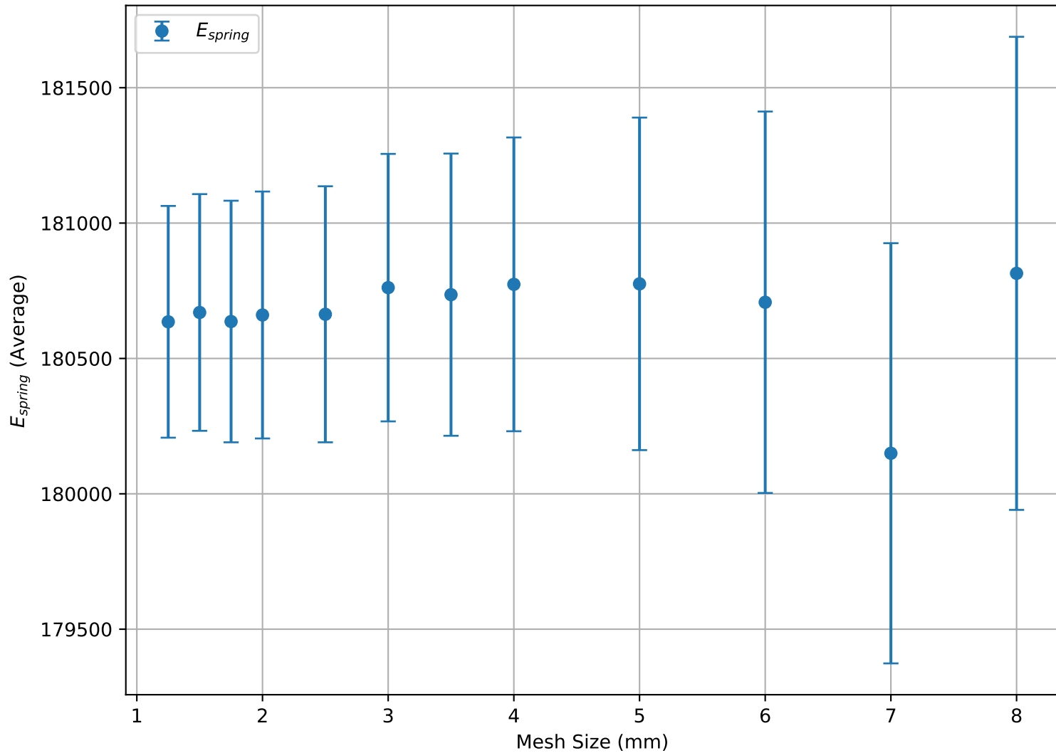
Average Spring Energy vs. Mesh Size, Displacement Control
