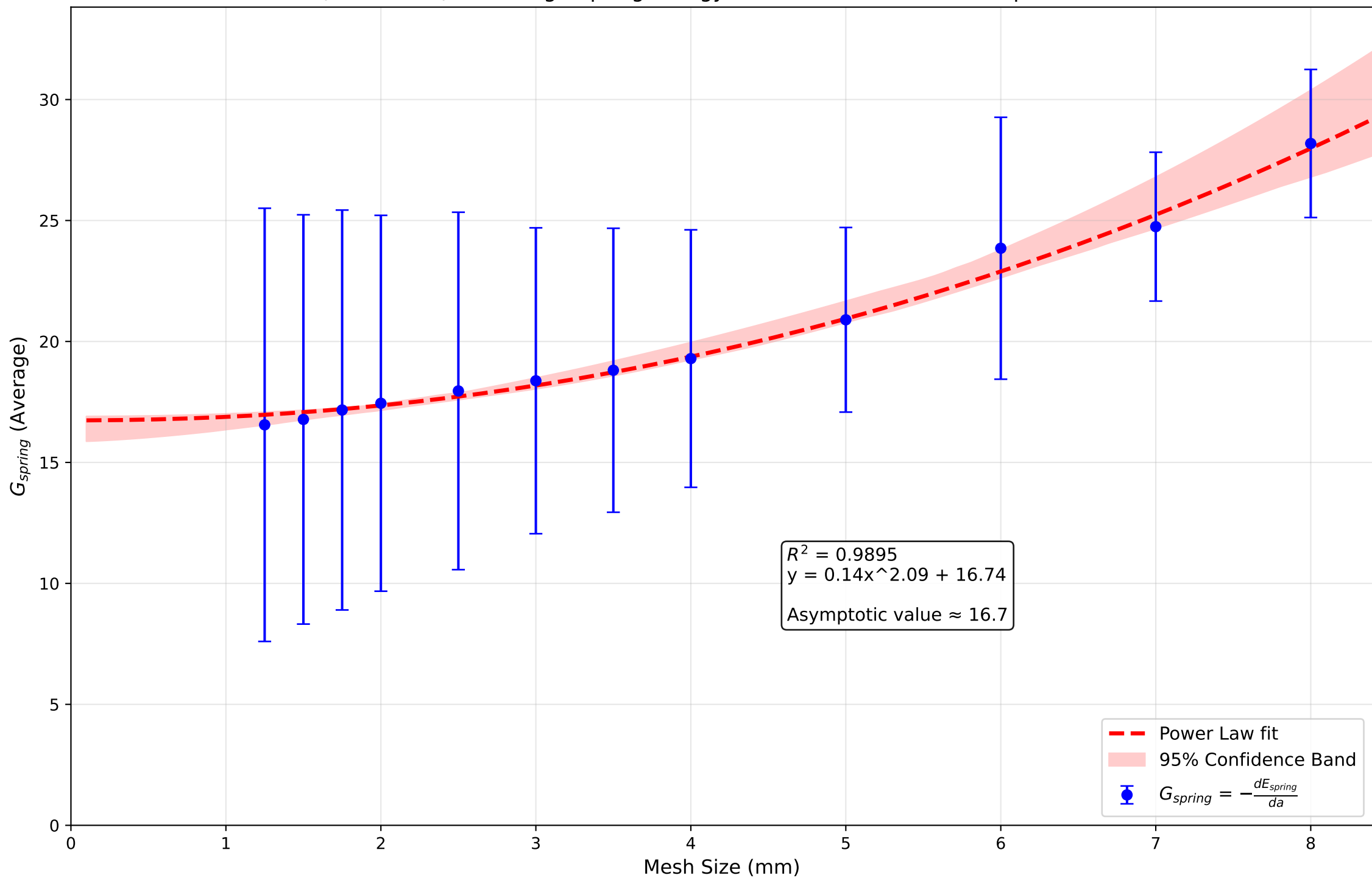
Best Fit (Power Law) of Average Spring Energy Gradient vs. Mesh Size Displacement Control
