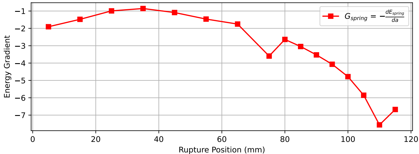
Gradient of Block Energies vs. Rupture Position
