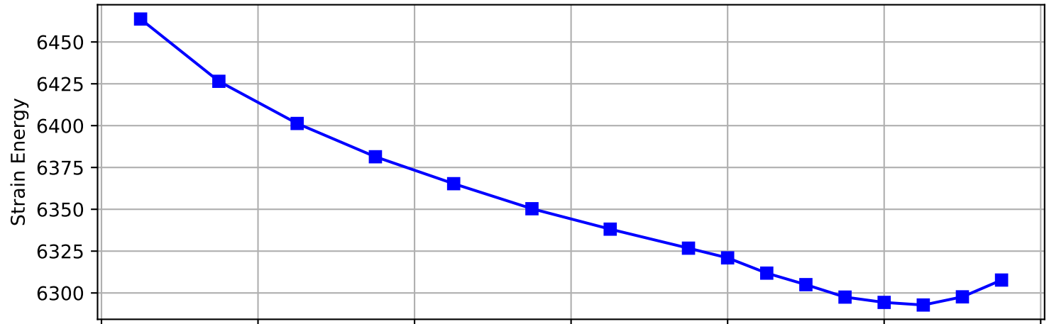
Side Block Energies vs. Rupture Position, Stress Control, 10.0MPa, 2.0mm
