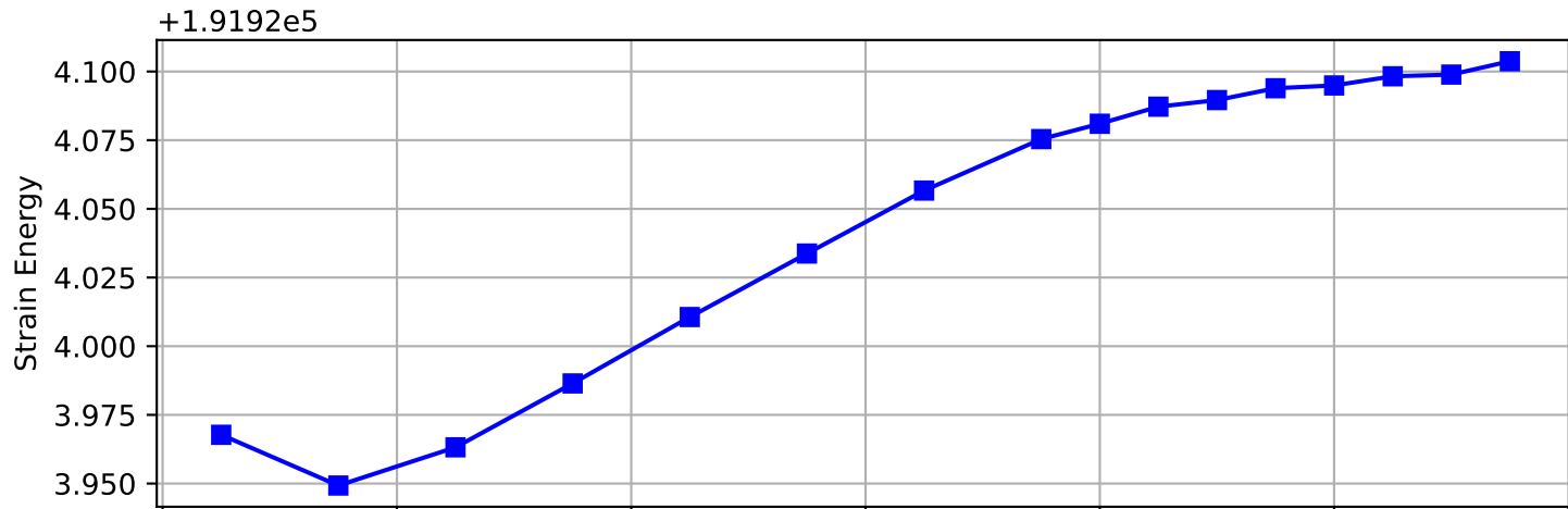
Gradient of Spring Energies vs. Rupture Position
