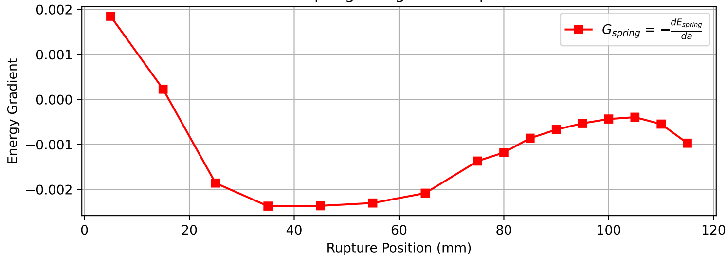
Gradient of Spring Energies vs. Rupture Position
