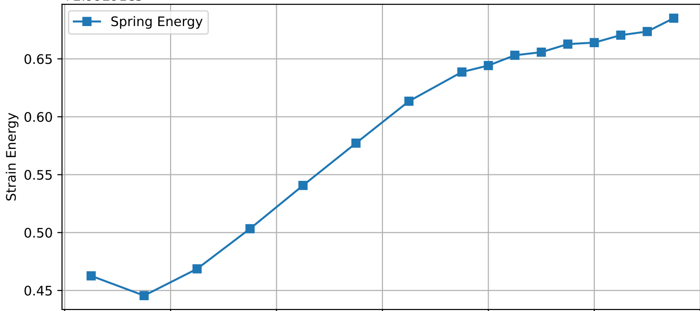
Spring Energy vs. Rupture Position, Displacement Control, 12.5MPa +2.99291e5
