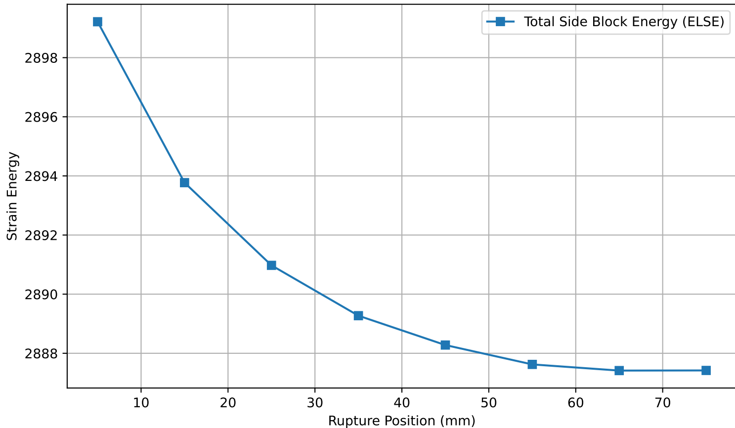
Strain Energy vs. Rupture Position
