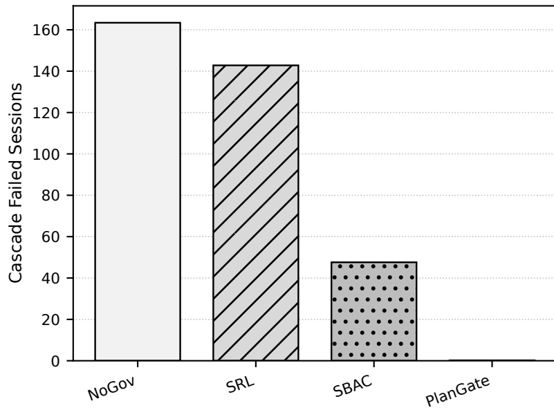
Core Mock Cascade Failure
