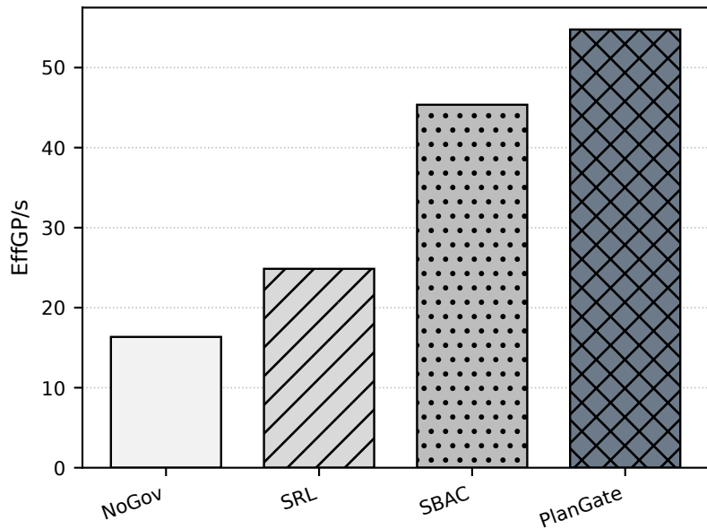
Core Mock Effective Goodput
