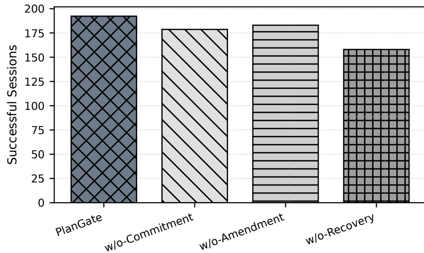
Recovery Success
