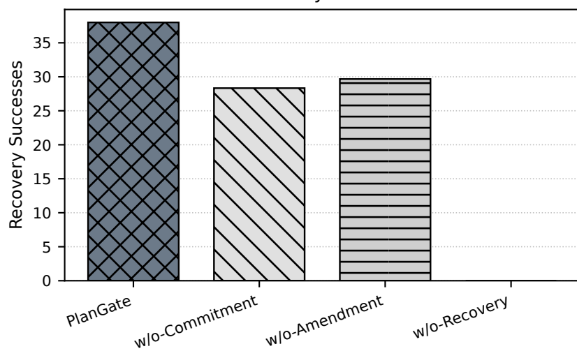
Recovery Success
