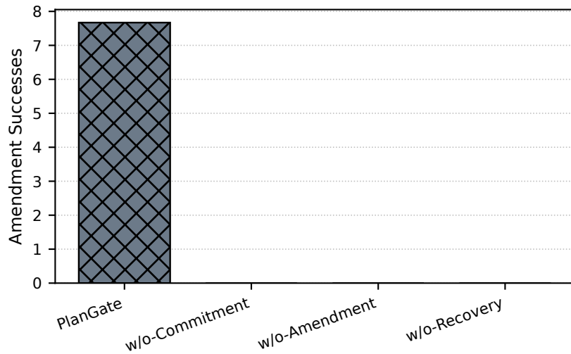
Amendment Success
