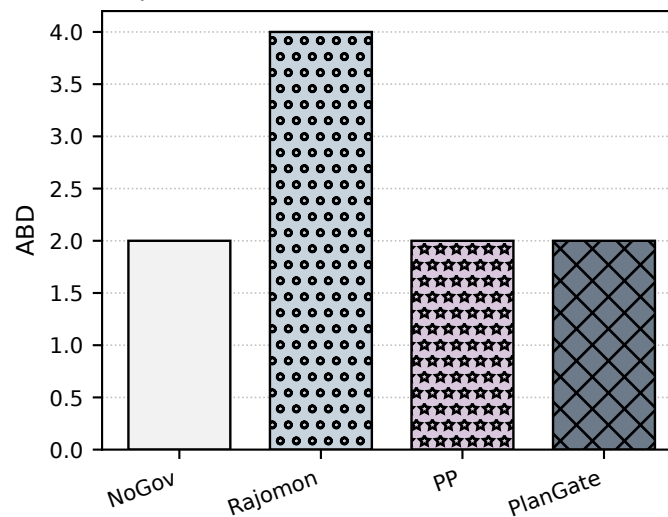
DeepSeek V4 Flash C5: Abandonment Burden
