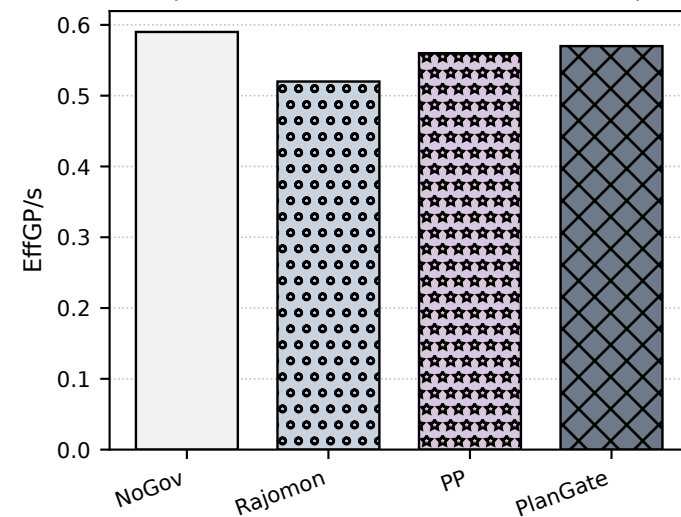
DeepSeek V4 Flash C5: Effective Goodput
