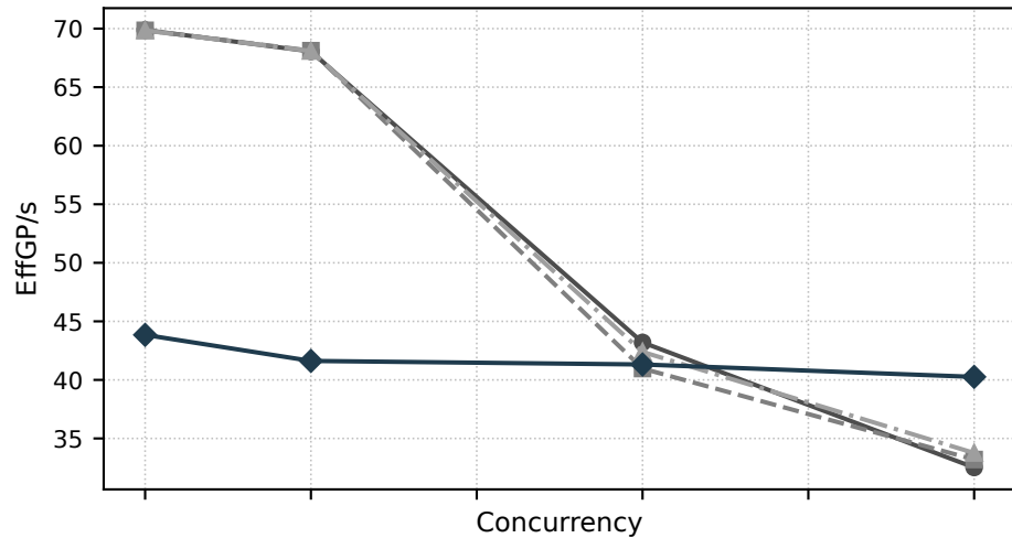
Exp6 ScaleConcReact Effective Goodput
