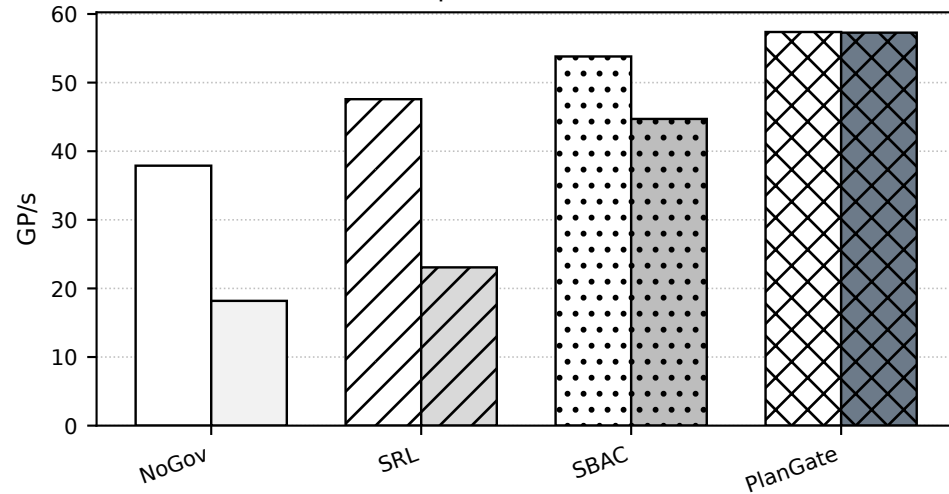
Exp10 Adversarial
