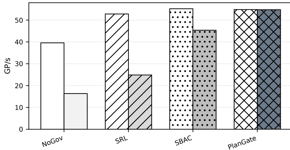
Exp6 ScaleConcReact
