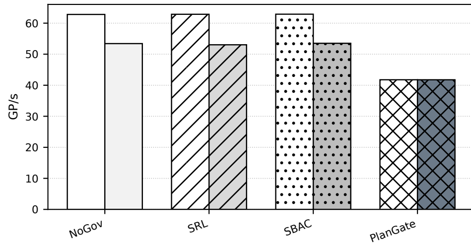
Exp10 Adversarial
