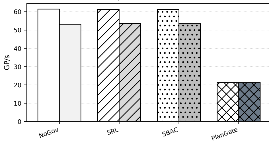
Exp6 ScaleConcReact
