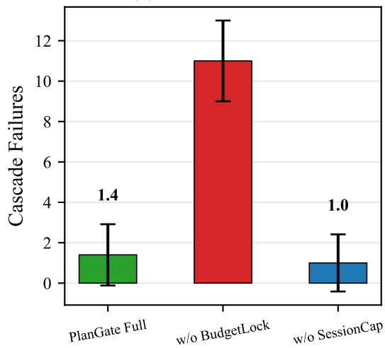
(b) Cascade Failures
