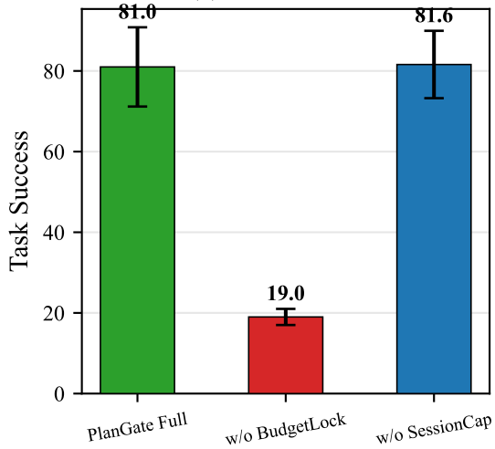
(a) Task Success
