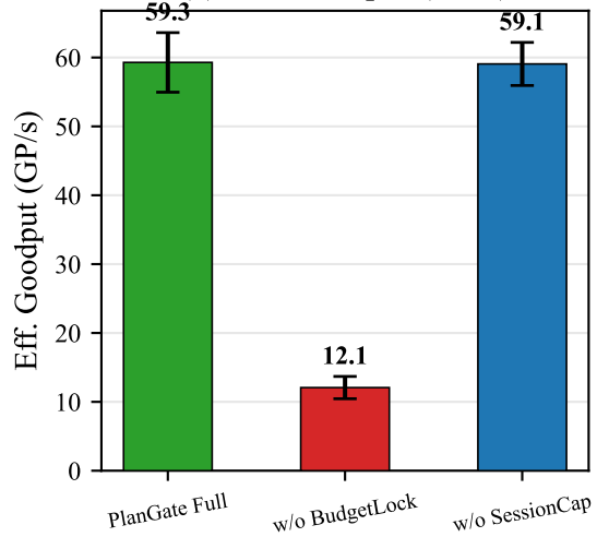
(c) Eff. Goodput (GP/s)
