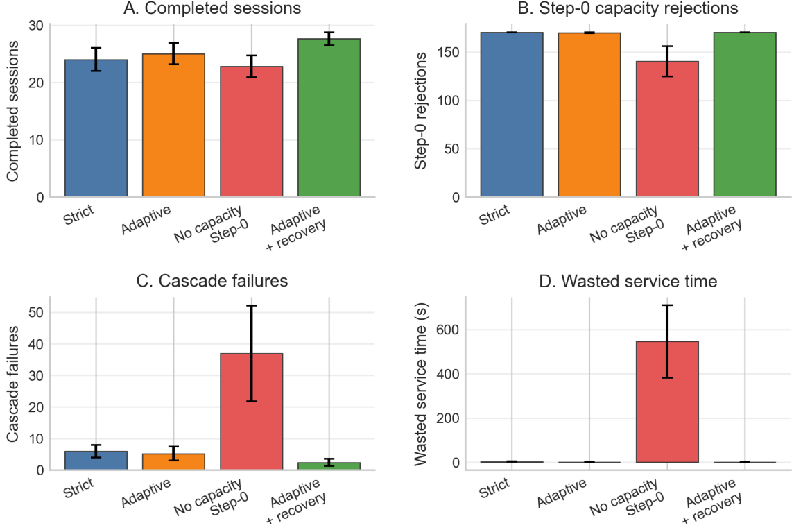
Business workflow trade-off at C=100 , F=0.2
