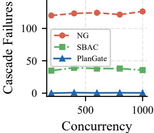
(a) Cascade Failures
