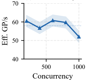
(b) PlanGate Goodput
