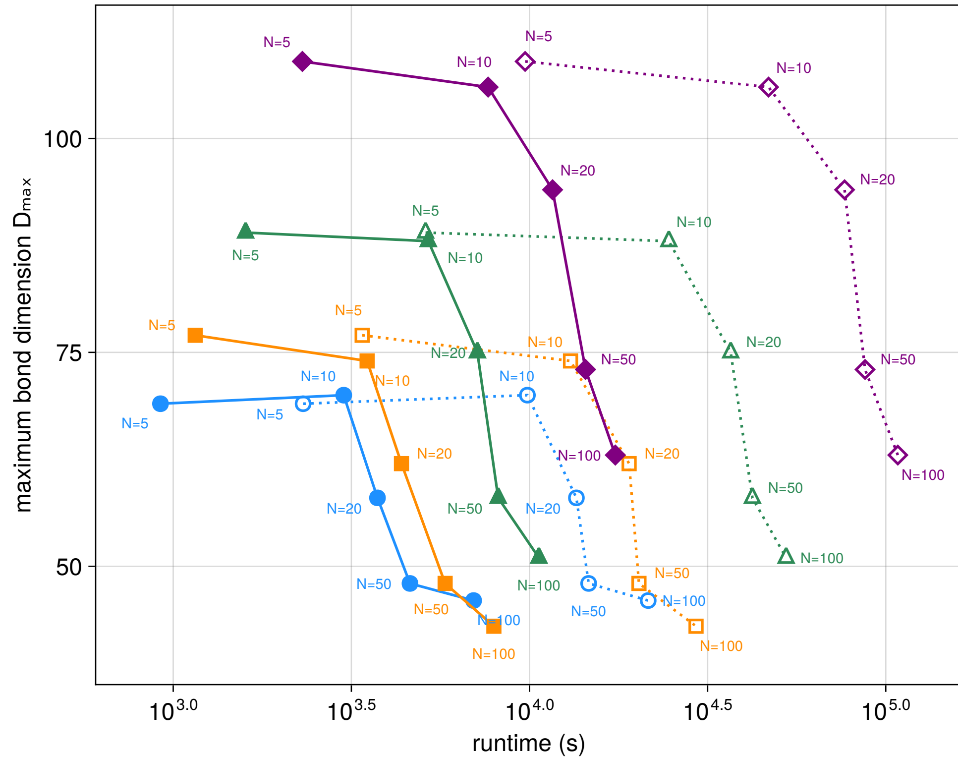
Spin-boson process tensor
