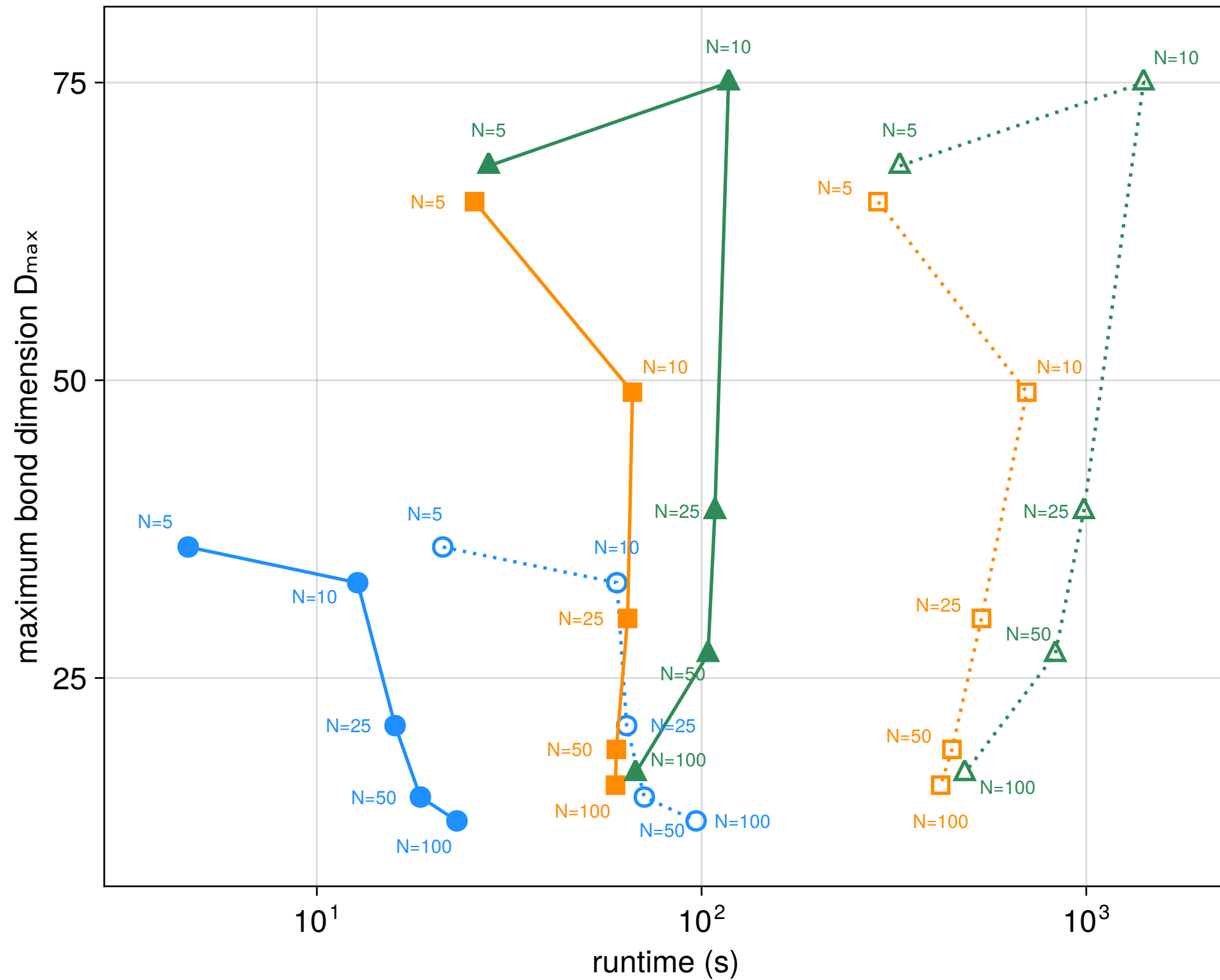
Central-spin process tensor
