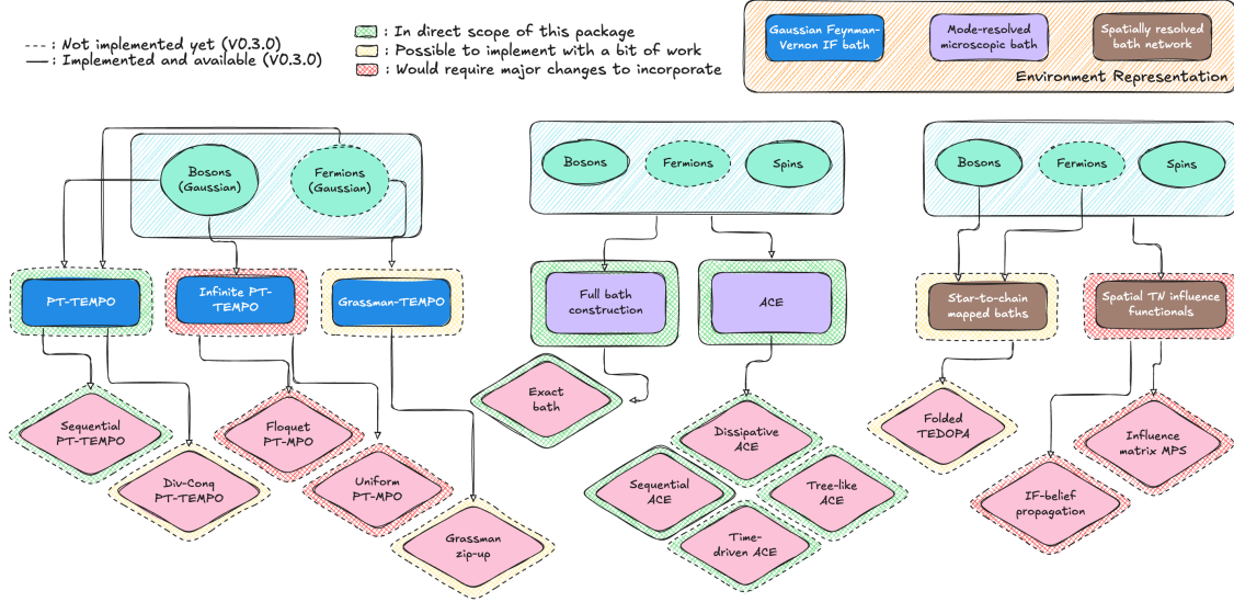
Figure 1: Overview of existing tensor-network routes to construct a process tensor. The diamonds identify construction and evaluation schemes or specialisations within these families; their roles are described in the text. Solid and dashed outlines distinguish whether a method is available in ProcessTensors.jl v0.3.0. Green, yellow, and red hatching indicate directions within the package’s direct scope, extensions requiring additional development, and approaches requiring major architectural changes, respectively. The branches show representative routes.
