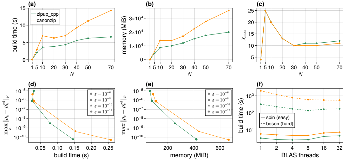
Figure 17: Comparison of the two ACE compression schedules. Panels (a)–(c) show median build time, total allocated memory, and maximum temporal bond dimension of the two compression schedules for the unpolarised central-spin scaling, benchmarked over seven samples. Panels (d)–(e) show trajectory error relative to a tightly converged reference. Panel (f) shows one benchmarked build per BLAS thread count for fixed spin (easy) and bosonic (hard) process tensors.
