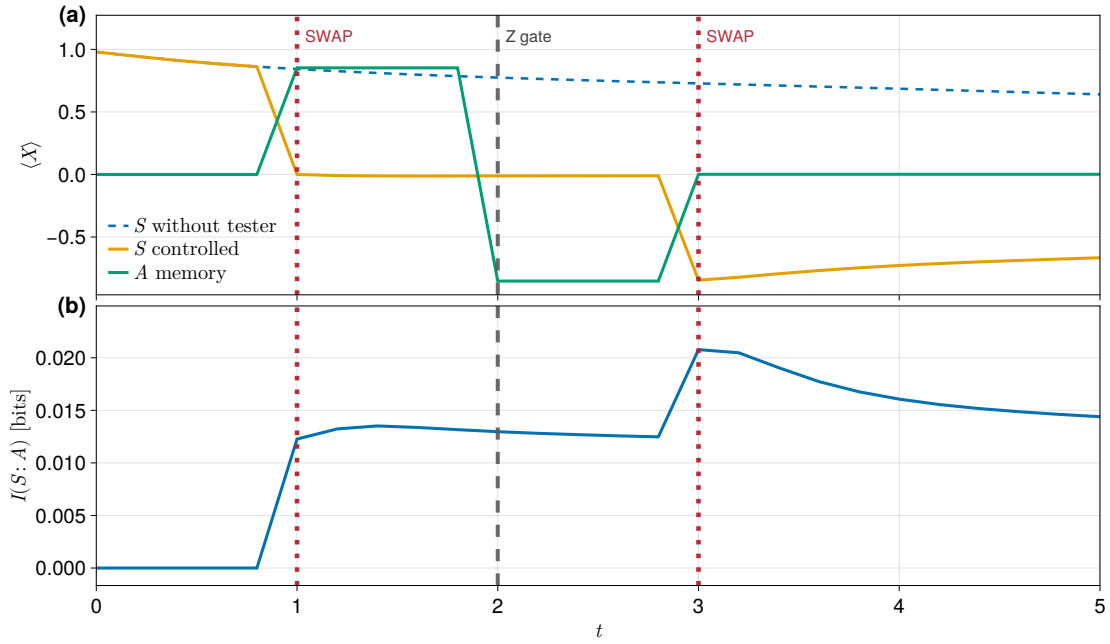
Figure 14: (a) Transverse magnetisation of the SWAP–phase–SWAP protocol. The first SWAP transfers \langle X \rangle from the noisy processor S to the isolated ancilla A , the Z_A gate reverses its sign, and the second SWAP returns it; the uncontrolled system continues to dephase on the processor. (b) System–ancilla correlation. The first SWAP parks the logical state in A while the environment retains the processor history; later evolution and the retrieval SWAP convert part of that history into I(S:A) \approx 0.02 bits. The small magnitude reflects the weak-coupling parameters used here.
