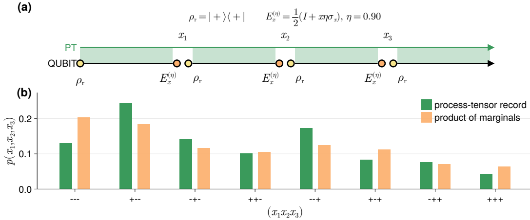
Figure 12: (a) Timeline of the Ramsey readout protocol. Three repeated readouts of the thermally dephasing qubit in Eq. (83), each followed by the same active reset, Eq. (85). The time exposed to the environment between each prepare and measure is the same for all three readouts. The green fill between the PT and QUBIT line depicts constant interaction between them. (b) Outcome-record probabilities p(x_1, x_2, x_3) . For some three-shot records the process tensor probabilities do not coincide with the products of the single-round marginals, indicating correlations between successive readouts.
