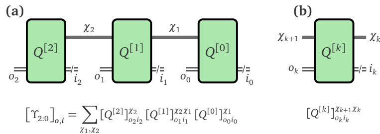
Figure 7: Matrix-product representation of a process tensor. (a) A three-step PT-MPO with time running from right to left: each core Q^{[k]} carries a pair of double-wired system legs (output o_k , input i_k ) and neighbouring cores are joined by a thick memory link \chi_k . (b) Index anatomy of a generic interior core. Open system legs mark the times at which operations may be inserted, while the horizontal bonds transmit the compressed influence of the environment between different parts of the experiment.
