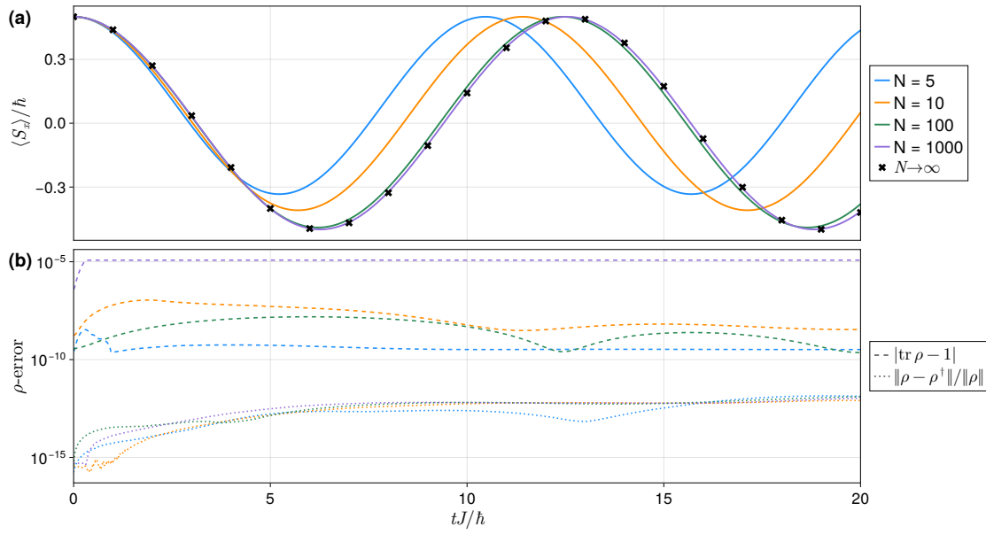
Figure 11: (a) Fully polarised central-spin dynamics. Reduced dynamics of the system spin coupled to a finite number of bath spins. Finite baths of the model in Eq. (81) approach the analytical N \rightarrow \infty precession in Eq. (82) as N increases. (b) Trace and hermiticity errors of \rho . The lower panel records |\text{Tr } \rho - 1| and \|\rho - \rho^\dagger\| / \|\rho\| .
