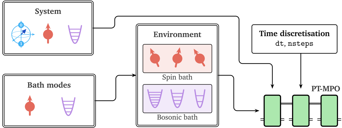
Figure 8: Microscopic ingredients of a ProcessTensor.
