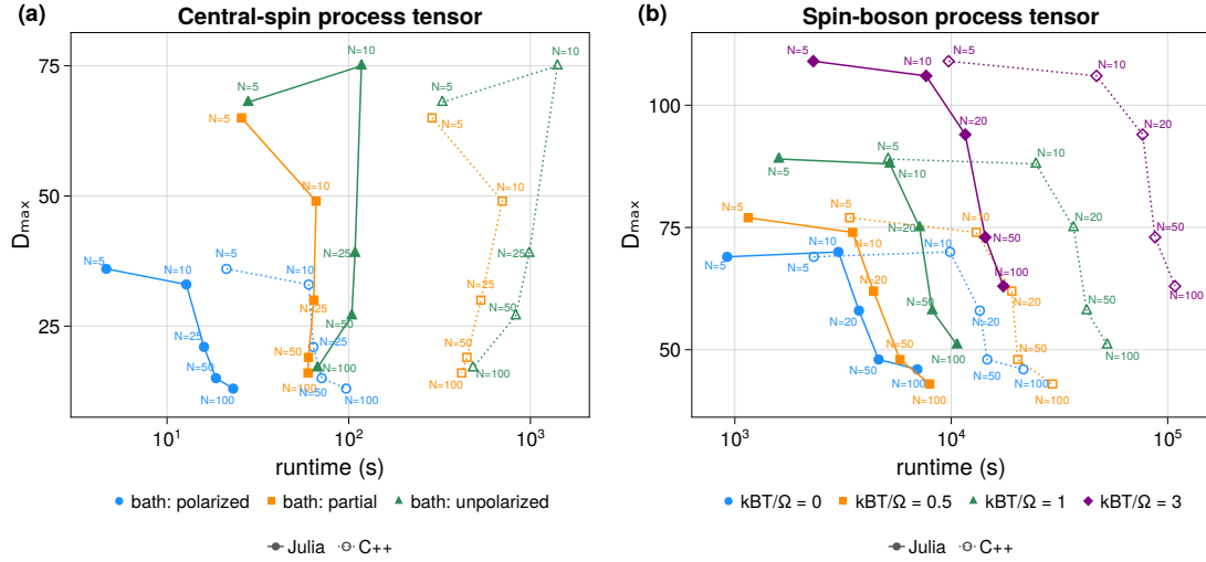
Figure 18: Benchmark of ProcessTensors.jl against the original C++ ACE toolkit. (a) Central-spin baths with fully polarised, partially polarised, and unpolarised initial states. (b) Lorentzian spin–boson baths at four different temperatures. Filled symbols denote Julia and open symbols C++; labels give the number N of bath modes. The horizontal axis is measured PT-MPO construction time and the vertical axis is the maximum internal bond dimension D_{\max} . Vertical alignment of matched points indicates equal retained bond dimension.
