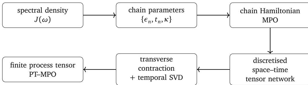
Figure 20: Prospective chain-mapping route from a continuum spectral density to a finite temporal PT-MPO.
