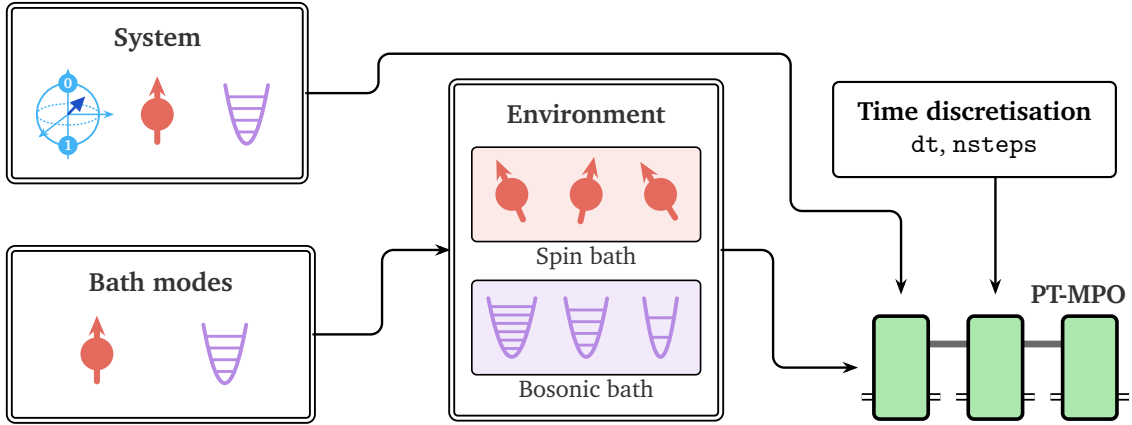
Figure 8: Microscopic ingredients of a ProcessTensor.
